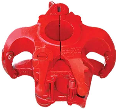
TI CODE: Drill Pipe Elevator 18° Bottleneck • G Series
